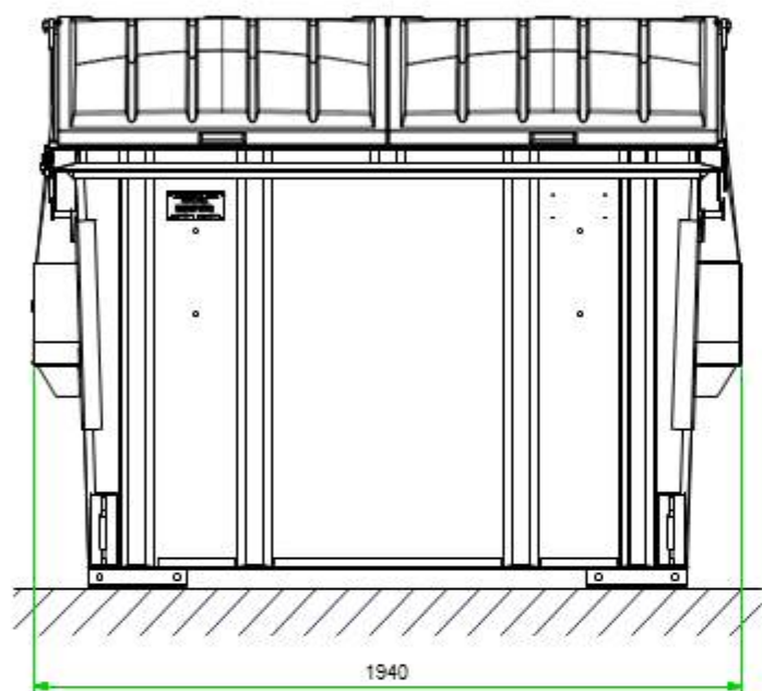
Frontlader F 5,0
